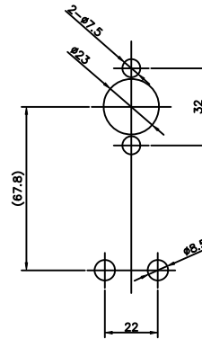
PANEL DRILLING DIMENSIONS.
