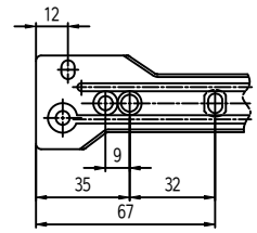
Cabinet member mounted 2mm from front edge
