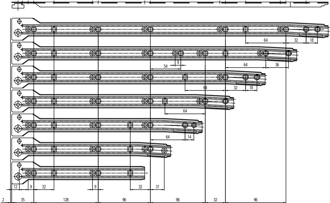
Selfclosing type drawerslide
