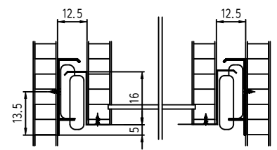
Rail width 1mm Installation width 12.5mm
