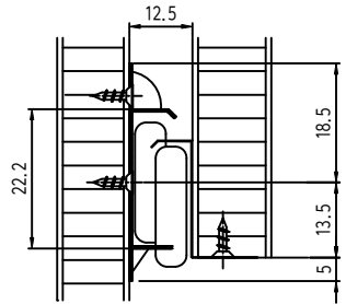
Bottom Mount
