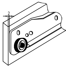
Cabinet member mounted 2mm from front edge
