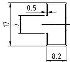
VIEW 'A' SCALE (2:1)
