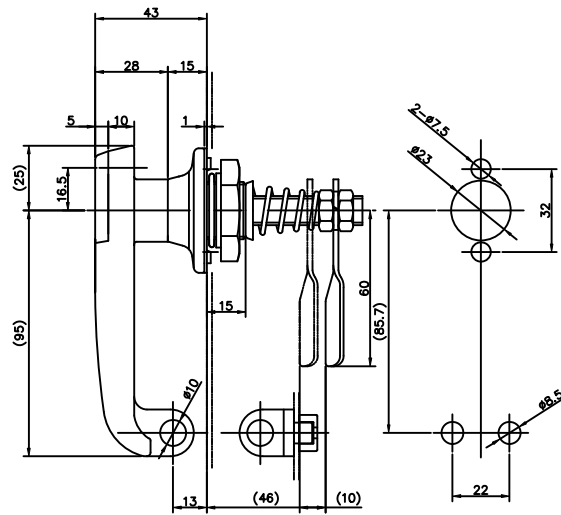
PANEL DRILLING DIMENSIONS.
