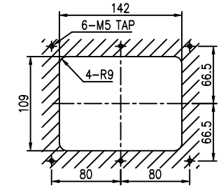
CUTTING HOLE (SCALE 1:2)
