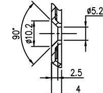
C.S.K DETAIL (SCALE 2:1)
